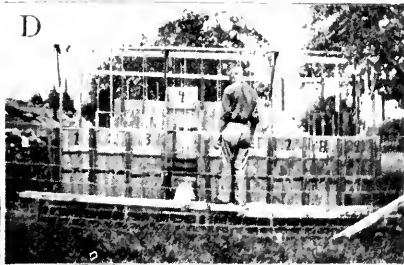
FIGURE 1. Multiple Choice Apparatus for Use with Pigs
